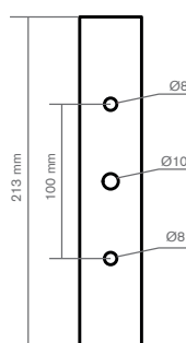
Bracket
