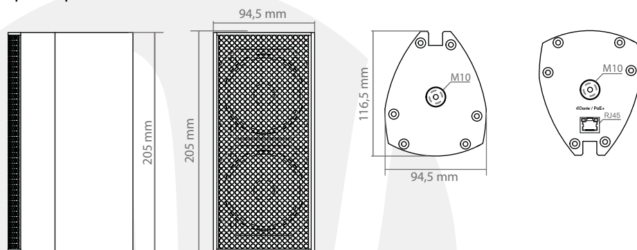
Spik 3 Mounting pole
